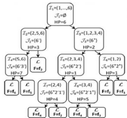
Figure 1. Illustration of the binary Search tree (BST).
