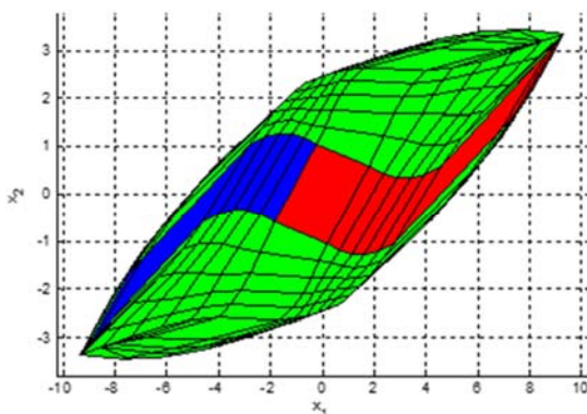
Figure 2. State space partition: polytopic sets \bar{R}_{sat} , \underline{R}_{sat} (green), R_{unsat} (blue and red).
