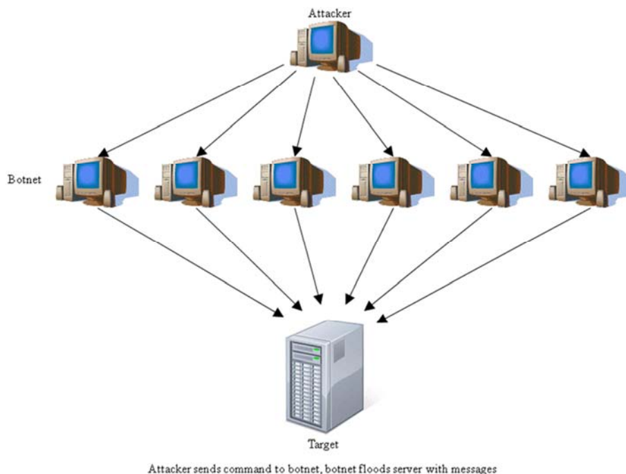
Figure 1. DDoS Attack.
