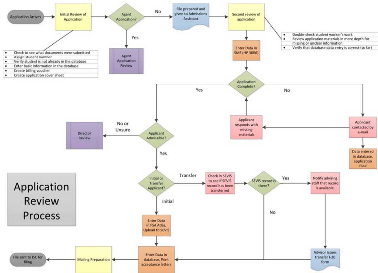
Figure 4. Workflow example.
