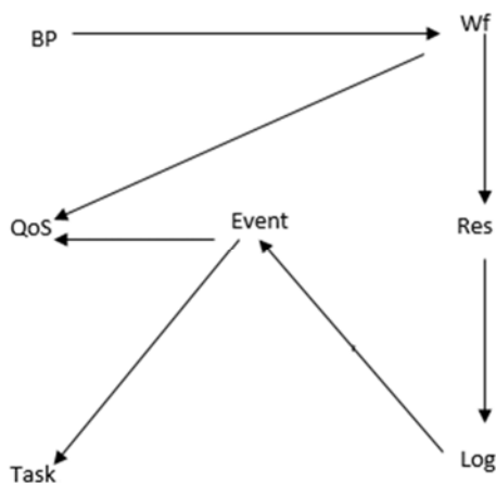
Figure 5. Commutative Diagram of main Concepts linked to the Business process.
