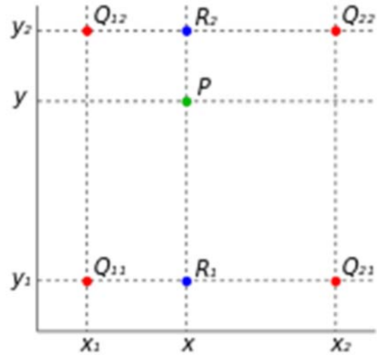
Figure 1. Bilinear Interpolation.
